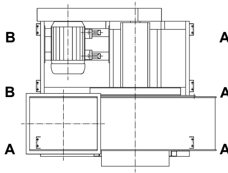
V-belt drive
