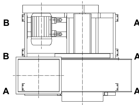
V-belt drive
